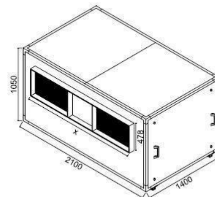
CFB 40 D 30.600 m 3 /h x 25 mmca 18 /18 duplex ventilador: 18 /18 duplex Otam motor: 10,0hp peso: 270Kg
